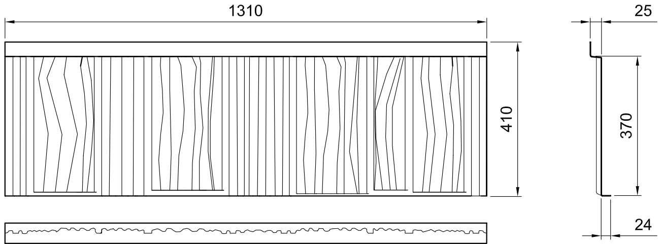
Figure 3.1 Shake Dimensions
