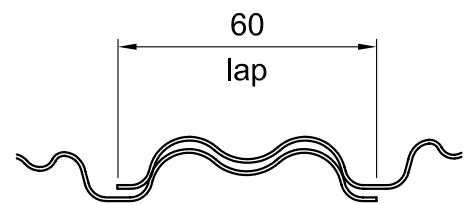
Figure 3.2 Nailing Detail
