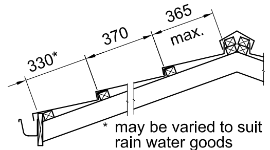
Figure 3.5 Batten Layout
