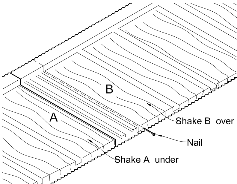
Figure 3.3 Overlap Detail
