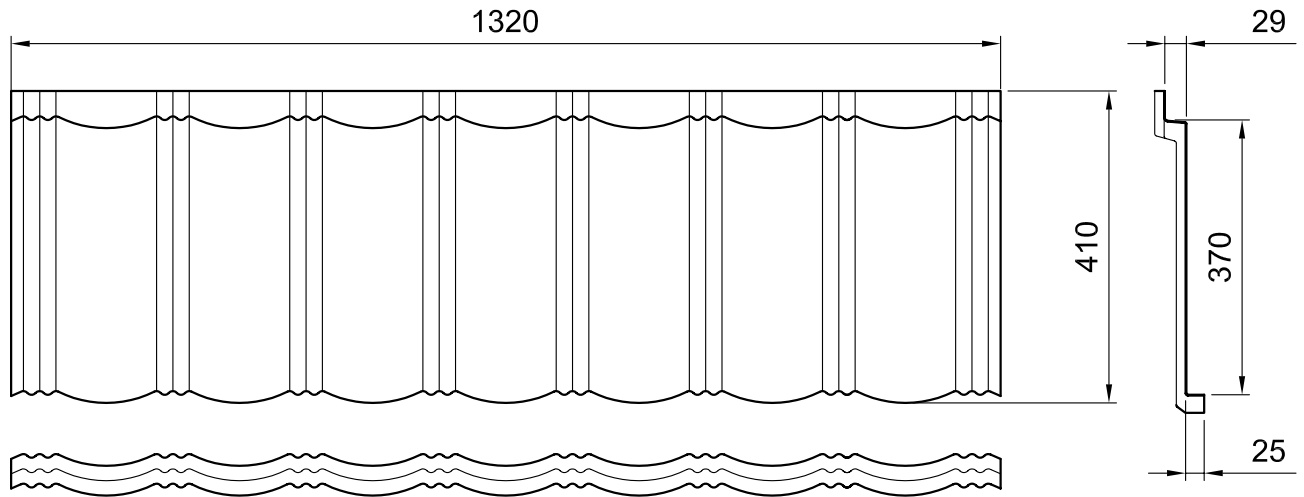
Figure 2.1 Tile Dimensions
