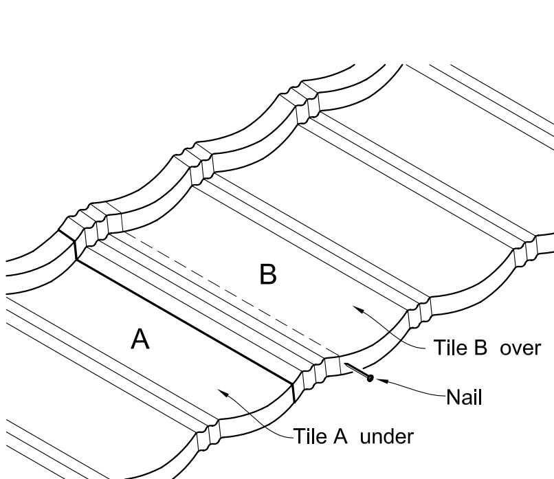
Figure 2.3 Overlap Detail
