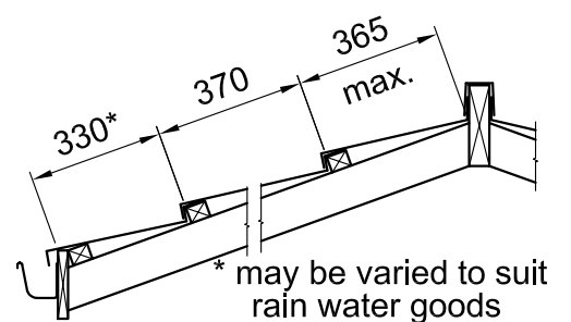
Figure 2.5 Batten Layout
