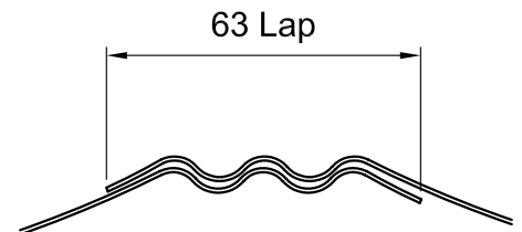
Figure 2.4 Lap Detail
