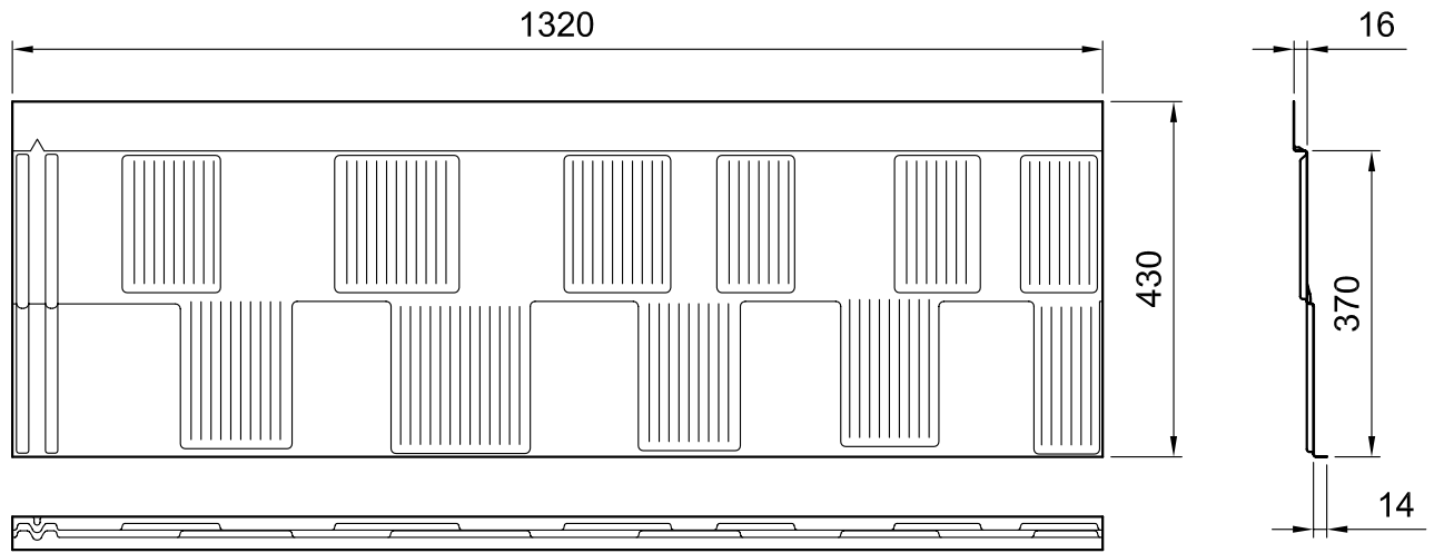
Fig 5.1 Shingle Dimensions
