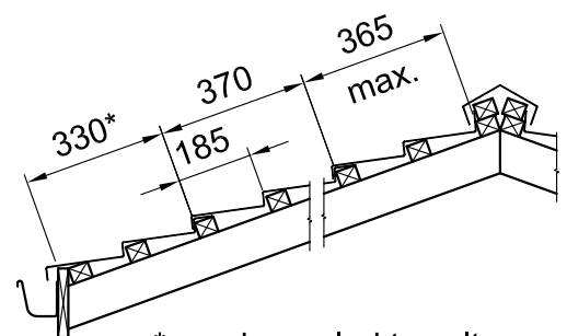
Figure 5.4 Lap Detail
