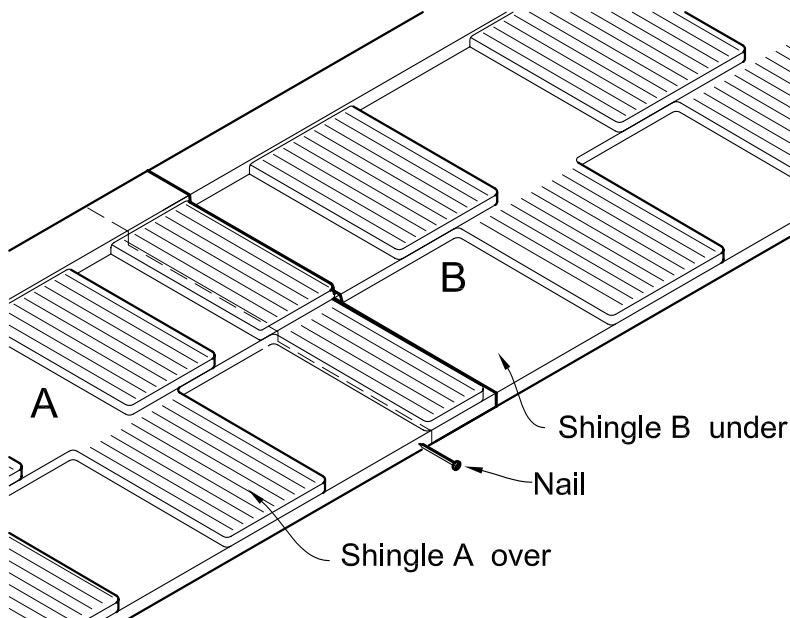
Figure 5.3 Overlap Detail
