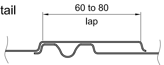
Figure 5.4 Lap Detail
