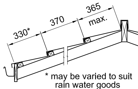
Figure 1.5 Batten Layout
