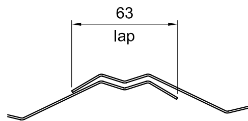
Figure 1.4 Lap Detail
