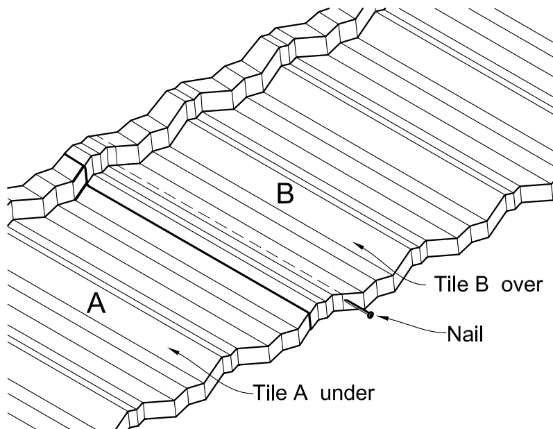
Figure 1.3 Overlap Detail
