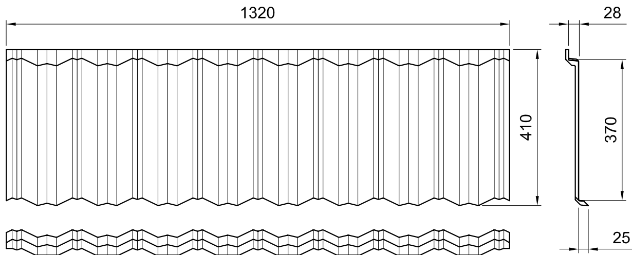
Figure 1.1 Tile Dimensions
